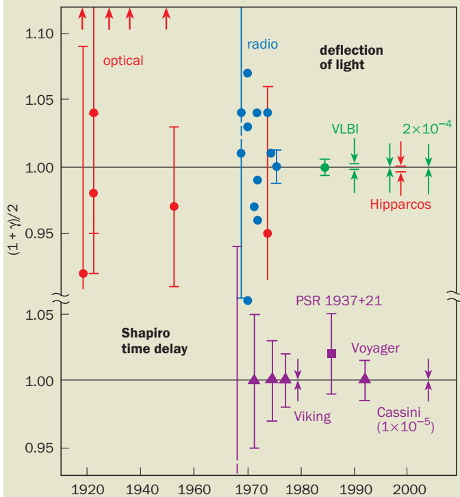
Einstein became a public celebrity when Arthur Eddington and colleagues measured the deflection of light by the Sun during the solar eclipse of 1919 and found that their results agreed with the predictions of general relativity. Measurements of the deflection (top) – plotted as (1 + \gamma)/2 , where \gamma is related to the amount of spatial curvature generated by mass – have become more accurate since 1919 and have converged on the prediction of general relativity: (1 + \gamma)/2 = 1 . The same is true for measurements of the Shapiro time delay (bottom). “Optical” denotes measurements made during solar eclipses (shown in red), with the arrows pointing to values well off the chart; “radio” denotes interferometric measurements of radio-wave deflection (blue); while Hipparcos was an optical-astrometry satellite. The left-most data point is the measurement made by Eddington in 1919, while the arrow just above it refers to the value obtained by his compatriot Andrew Crommelin (see “Einstein and the eclipse” on page XX). The best deflection measurements (green) are accurate to 2 parts in 10^4 and were obtained with Very Long Baseline Radio Interferometry (VLBI; see Shapiro et al. in further reading). A recent measurement of the Shapiro time delay by the Cassini spacecraft, which was on its way to Saturn, was accurate to 1 part in 10^5 (see Bertotti et al. in further reading).
