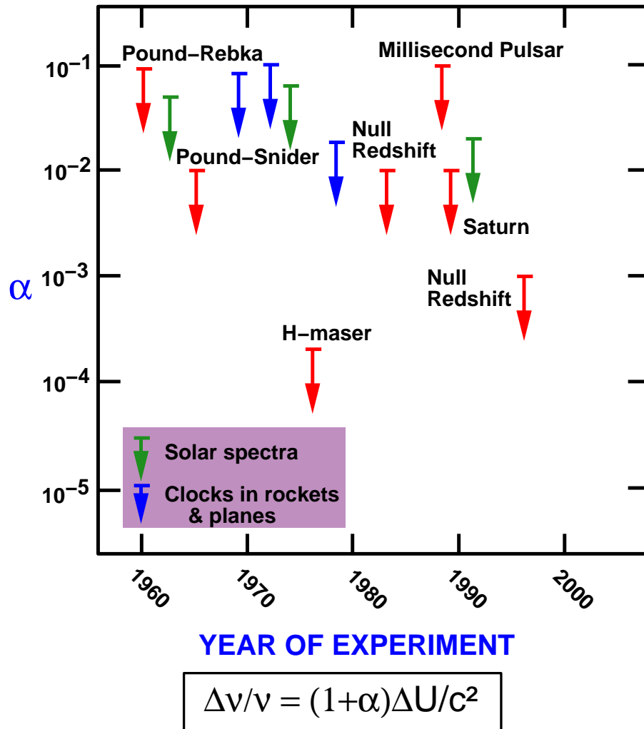
Fig. 3. Selected tests of local position invariance via gravitational redshift experiments, showing bounds on \alpha , which measures degree of deviation of redshift from the formula \Delta\nu/\nu = \Delta U/c^2 .
